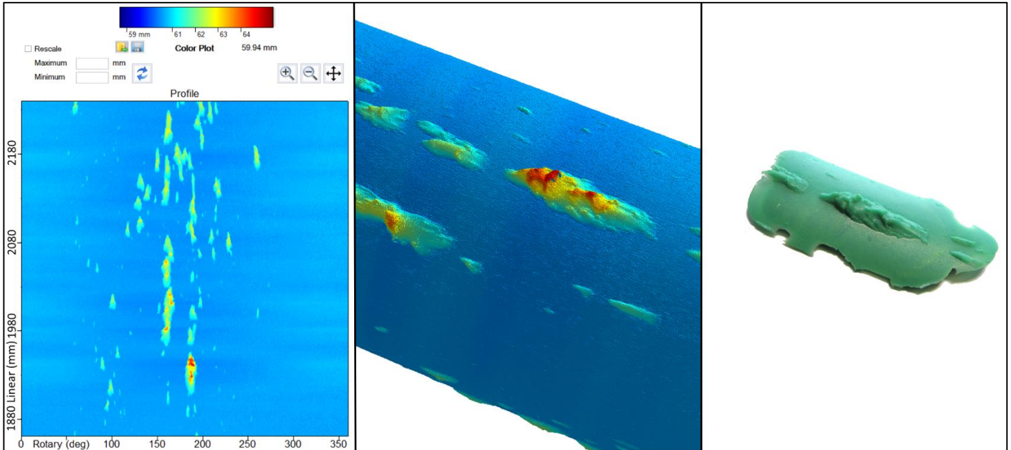
Pitting features shown in a section of 120mm smoothbore cannon. From Left: Laser Profile Data [Plan View]. LaserViewer™ 3D, Rubber Replica
