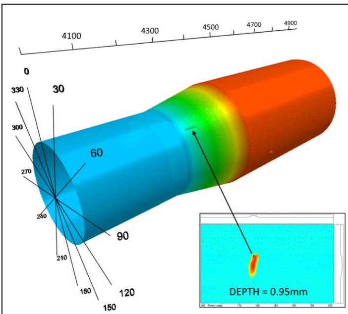
120mm barrel section with feature and axial labels displayed
